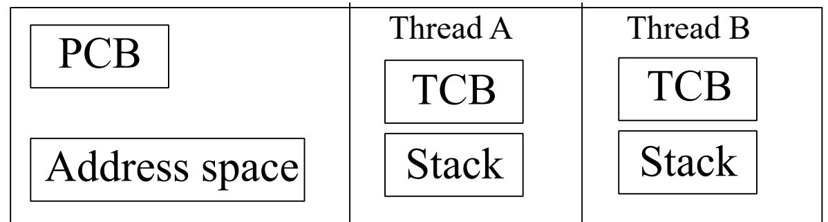
Modello multithreading
