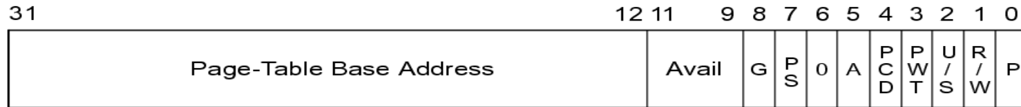
Page-Directory Entry (4-KByte Page Table)
