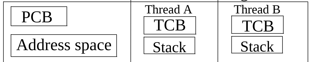
Modello multithreading
